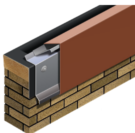
TerminEdge One Fascia Single-Ply
