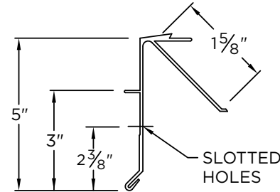
EXTRUDED PROFILE
